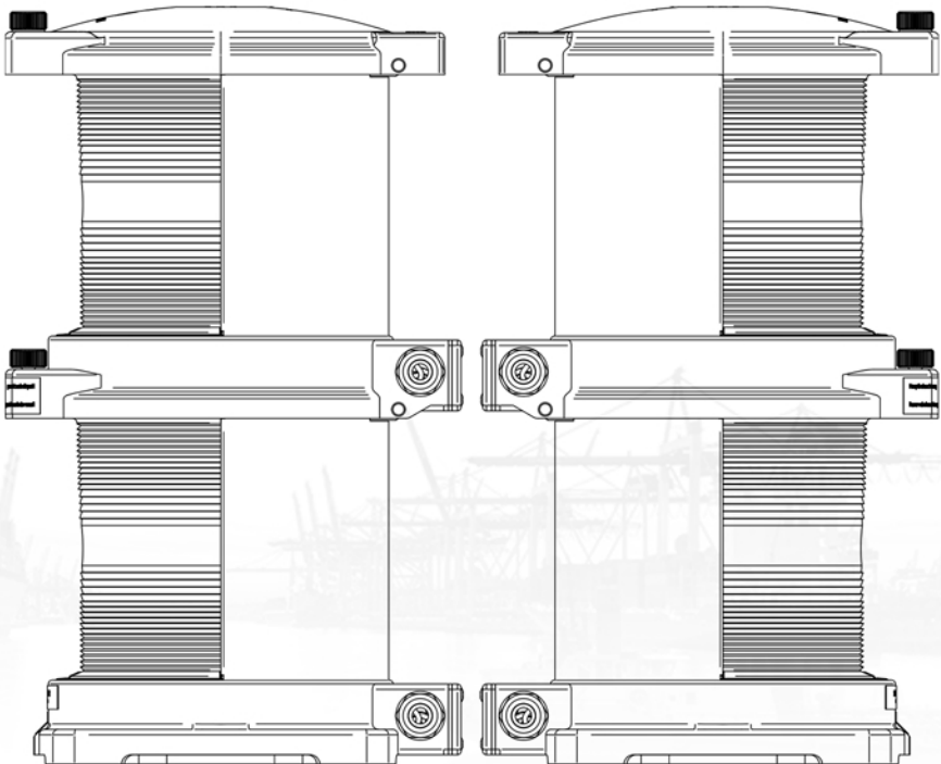
180° double lantern (see table below)
